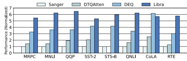
Fig. 10: Comparison of performance between Libra and other accelerators. All results are normalized to Sanger.
