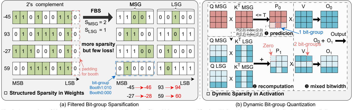
Fig. 3: An overview of bit-group-based algorithm. (a) Libra takes filtered bit-group sparsification (FBS) to balance weight distribution with negligible accuracy loss. (b) Libra employs dynamic bit-group quantization (DBQ) to introduce dynamic sparsity in activations.
