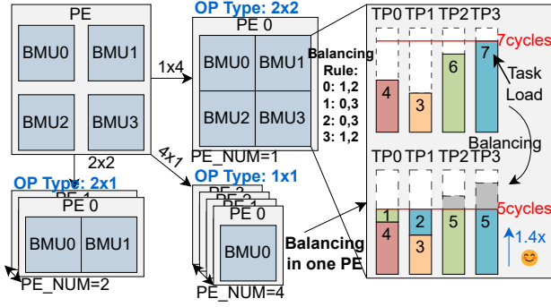
Fig. 6: Cases of adaptive bit-width in PE. Workload balancing within PE for 2x2 OP type.
