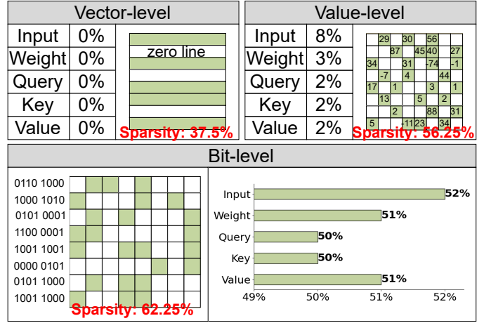
Fig. 2: Preliminary experimental results on the vector-level, value-level and bit-level sparsity in the BERT model and GLUE dataset.
