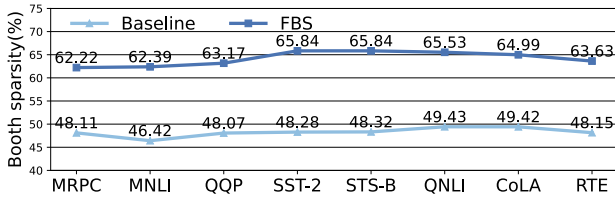
Fig. 7: Average Booth sparsity of linear layer weights across different tasks on Glue.
