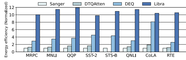
Fig. 11: Comparison of energy efficiency between Libra and other accelerators. All results are normalized to Sanger.
