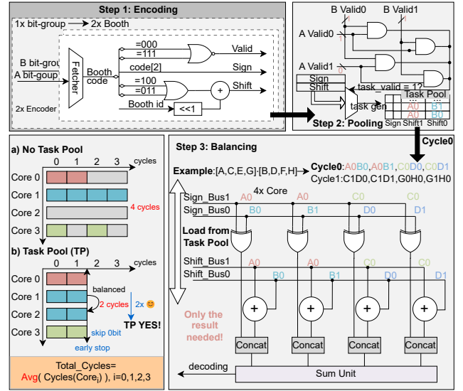
Fig. 5: Illustration of workload balancing in BMU via task pool.
