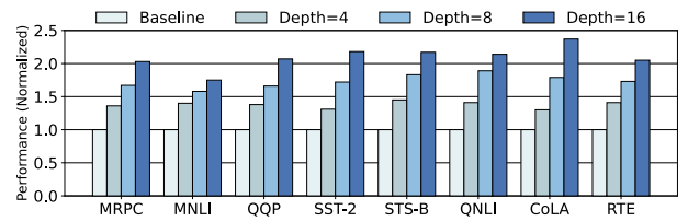
Fig. 9: Performance analysis with different task pool depths. All results are normalized to Baseline (depth=0).
