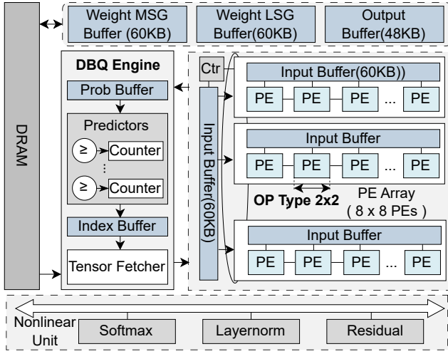
Fig. 4: Overview of Libra hardware architecture.
